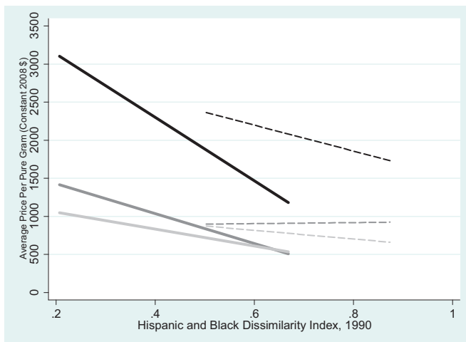
Fig. 6. Lines of best fit for the relationship between heroin price and segregation. Black lines indicate the average price per pure gram, 1990–1992. The dark grey lines indicate the average price per pure gram, 1993–2000. The light grey lines indicate the average price per pure gram, 2001–2008. Solid lines are Hispanic segregation and dashed lines are black segregation.
